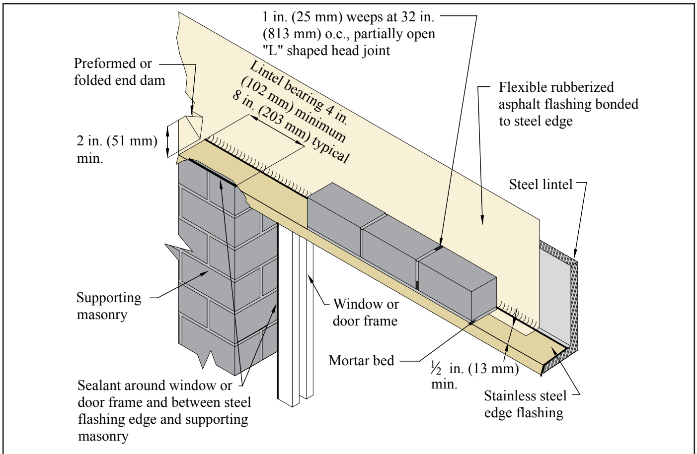
Figure 2—Steel Lintel Flashing Detail (ref. 8) (backing not shown for clarity)
