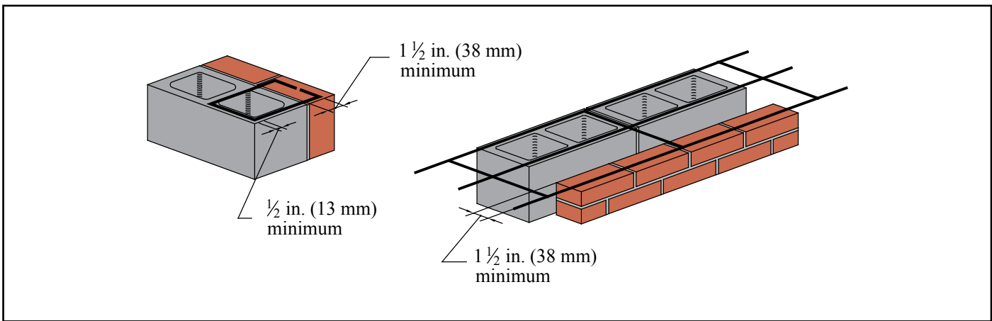
Figure 6—Minimum Embedment of Joint Reinforcement and Wire Ties
