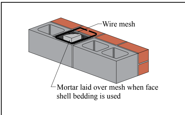
Figure 7—Use of Mesh to Facilitate Embedment of Anchor in Mortar
