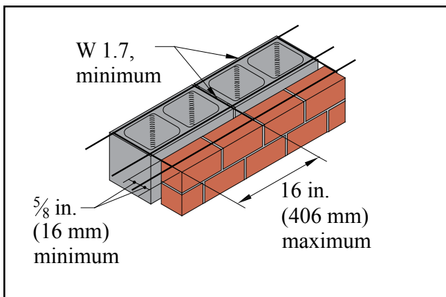
Figure 5—Requirements for Joint Reinforcement Used to Anchor Veneer
